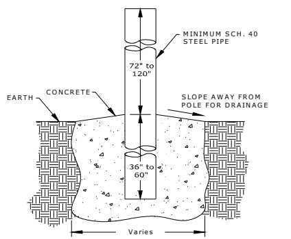
POLE INSTALLATION DETAIL
